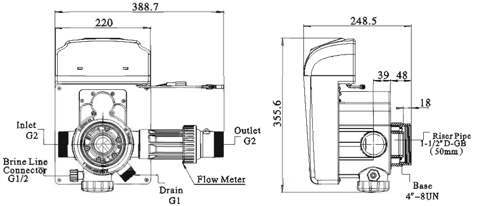
Structure Chart of N74A3 ( 63610 )
