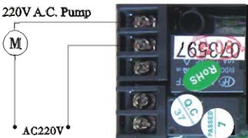
Figure 3-7Wiring of Booster Pump on Inlet
