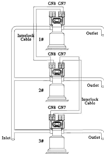
Figure 3-12 Interlock system
