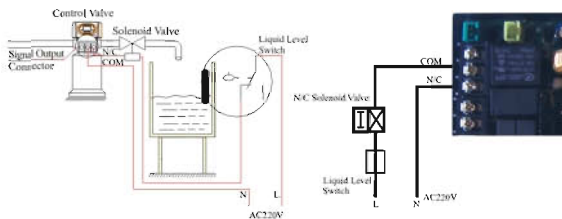
Figure 3-1 Wiring of Solenoid Valve on Outlet
