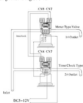
Figure 3-13 Series system
