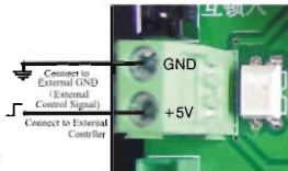
Figure 3-11 Wiring of Remote Input
