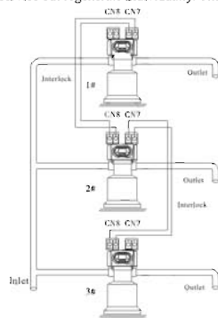
Figure 3-12 Interlock system
