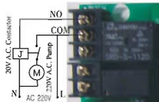
Figure 3-8 Wiring of Booster Pump on Inlet
