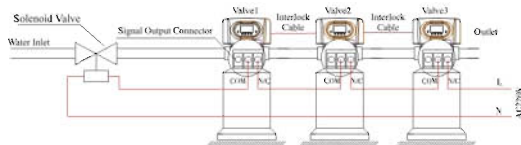
Figure3-4 Wiring of Solenoid Valve in Inlet
