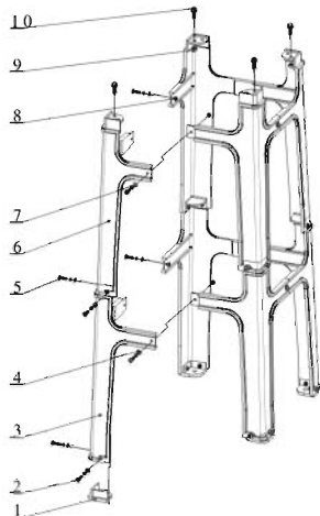
5040009 Seat frame Assembly &amp; Parts:
