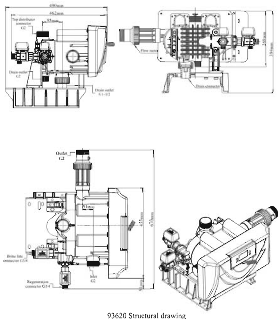
93620 Structural drawing
