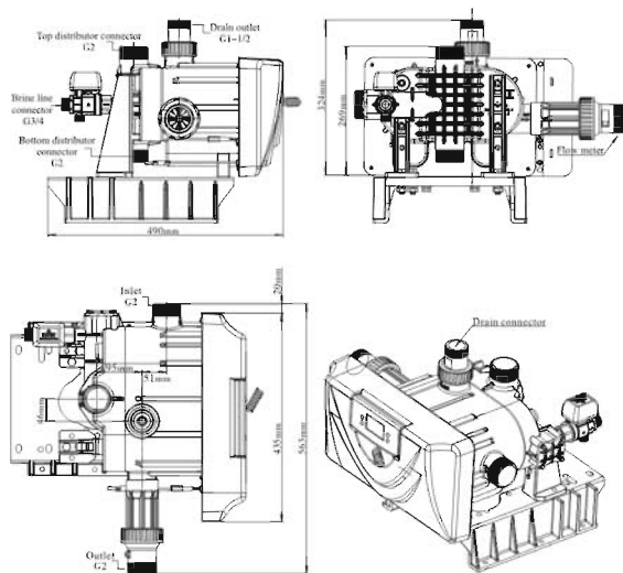
63620 Structural drawing
