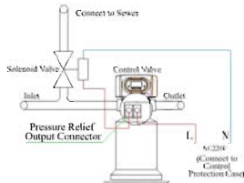
Figure 3-10 Wiring of Pressure Relief Output
