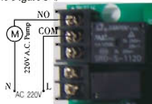
Figure 3-7 Wiring of Booster Pump on Inlet
