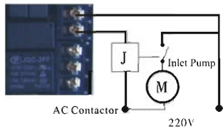
Figure3-17 Wiring of Soft Water Pump Power More Than 1KW
