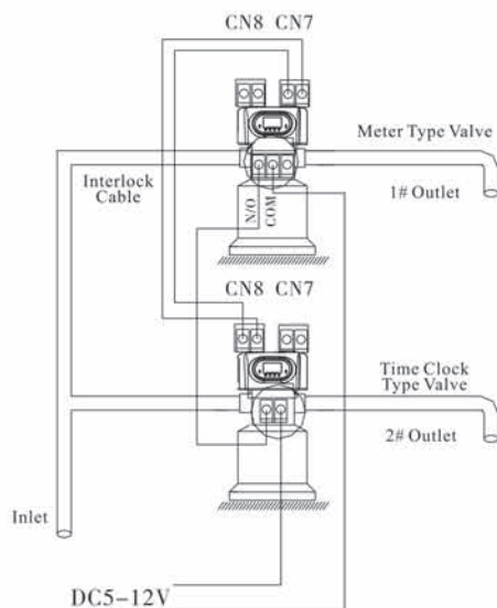
Figure 3-13 Series system
