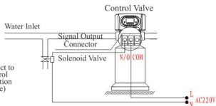
Figure3-3 Wiring of Solenoid Valve on Pressure Relief Port
