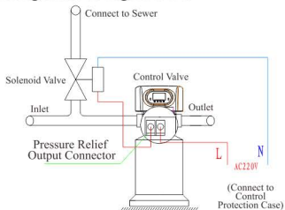
Figure 3-10 Wiring of Pressure Relief Output
