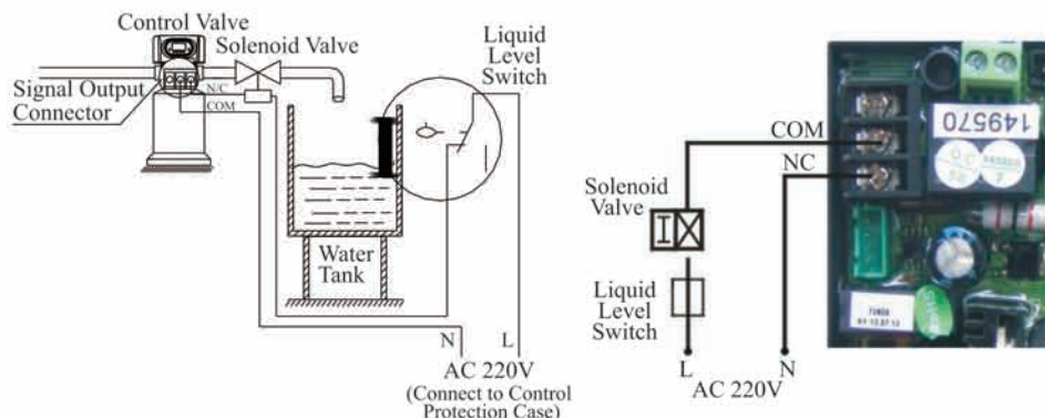
Figure 8 Wiring of Solenoid Valve on Outlet
