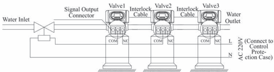
Figure 10 Wiring of Solenoid Valve in Inlet
