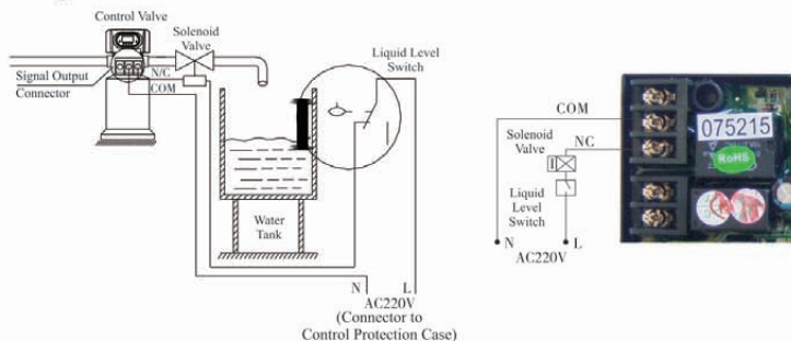
Figure 3-1 Wiring of Solenoid Valve on Outlet
