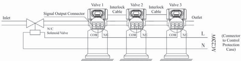
Figure 3-4 Wiring of Solenoid Valve on Inlet
