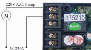
Figure 3-7 Wiring of Booster Pump on Inlet
