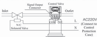
Figure 3-2 Wiring of Solenoid Valve on Inlet
