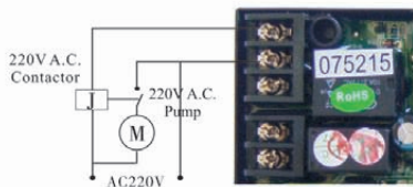
Figure 3-8 Wiring of Booster Pump on Inlet
