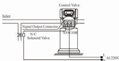
Figure 3-3 Wiring of Pressure Relief Connector
