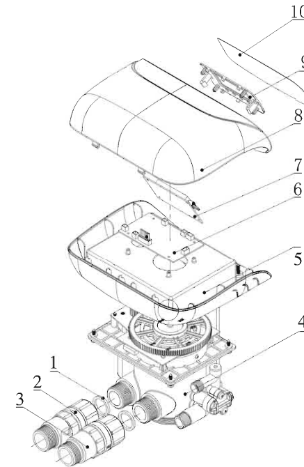
F82AG-LCD/F82BG-LCD Spare Part and Part Number
