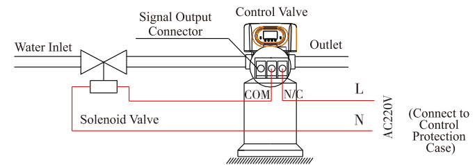
Figure 3-2 Wiring of Solenoid Valve on Inlet
