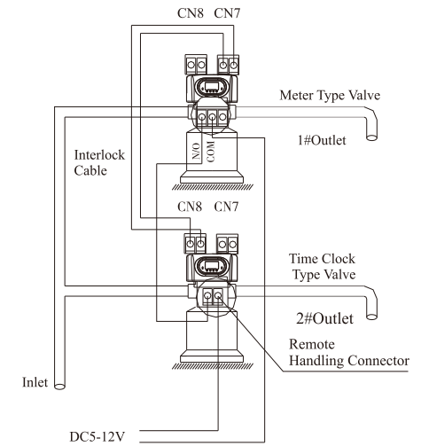
Figure 3-11 Series system
