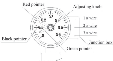
Schematic diagram of pressure gauge
