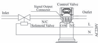
Figure 3-3 Wiring of Solenoid Valve on Inlet
