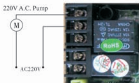
Figure 3-7Wiring of Booster Pump on Inlet
