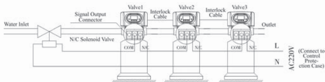
Figure 3-4 Wiring of Solenoid Valve in Inlet
