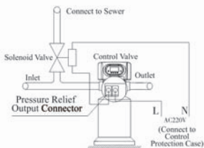
Figure 3-10 Wiring of Pressure Relief Output
