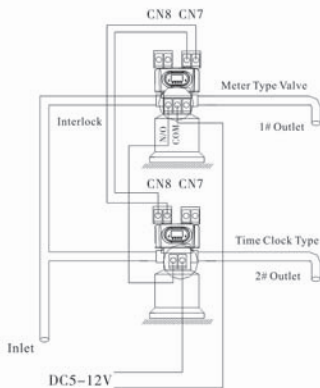
Figure 3-13 Series system
