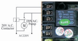
Figure 3-8 Wiring of Booster Pump on Inlet
