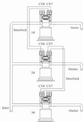
Figure 3-12 Interlock system
