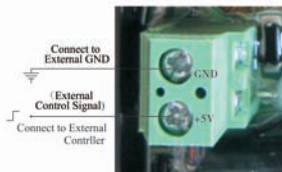
Figure 3-11 Wiring of Remote Input
