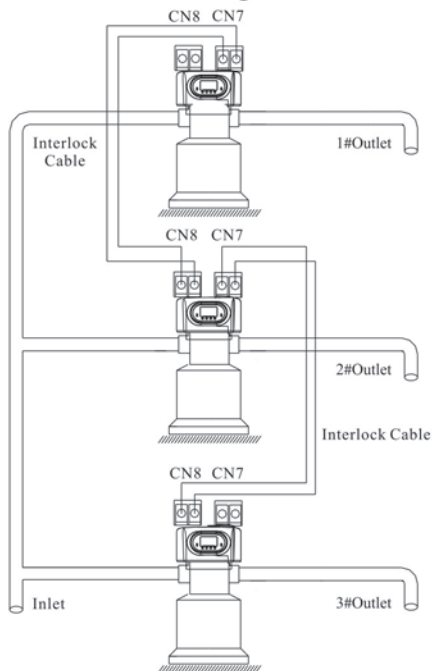
Figure 3-12 Interlock System
