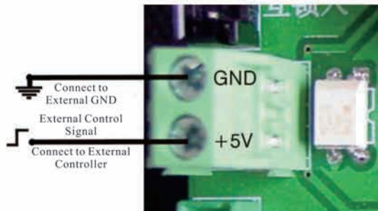
Figure 3-11 Wiring of Remote Input
